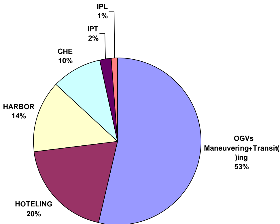
Figure 19: Distribution of Diesel PM Emissions by Source Categories for POLA and POLB in 2002
