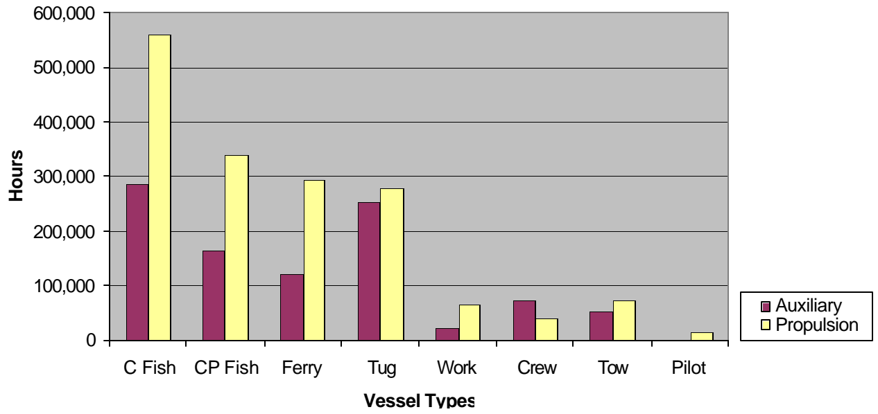
Figure 7: Total Engine Hours of Operation Per Year
