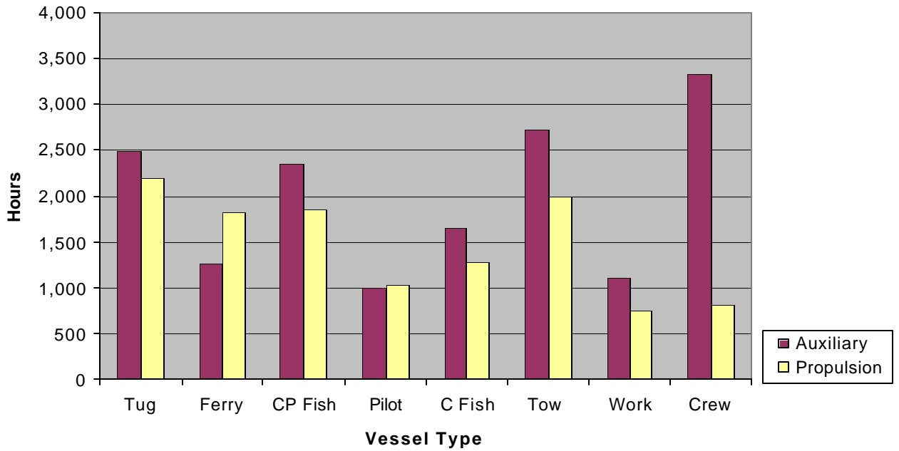
Figure 6: Average Engine Hours of Operation Per Year
