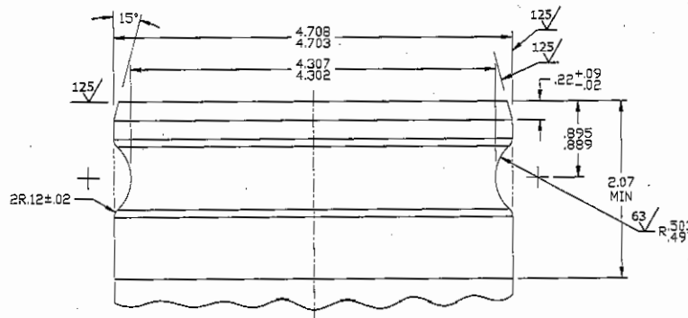
Figure 3B Phase I Vapor Recovery Adaptor Cam and Groove Specification
