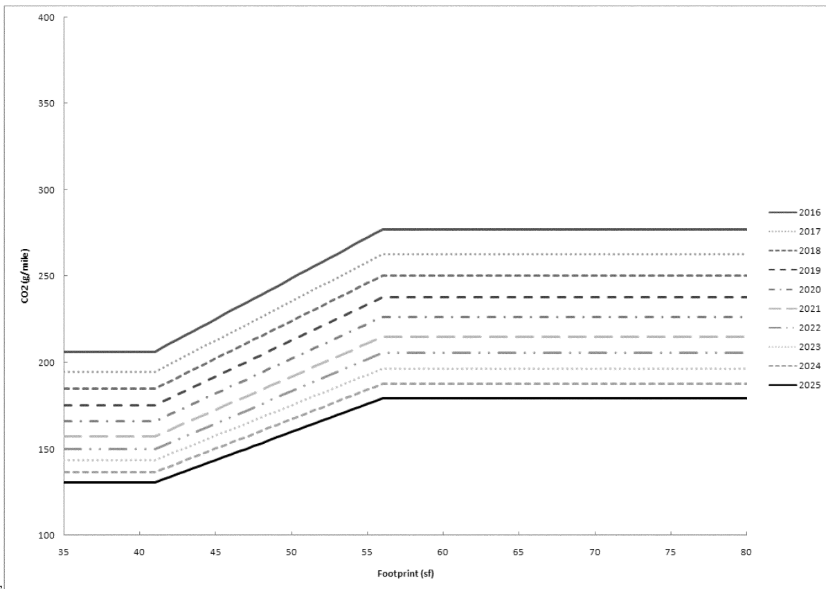
Figure I- 3 CO2 (g/mile) Passenger Car Standards
