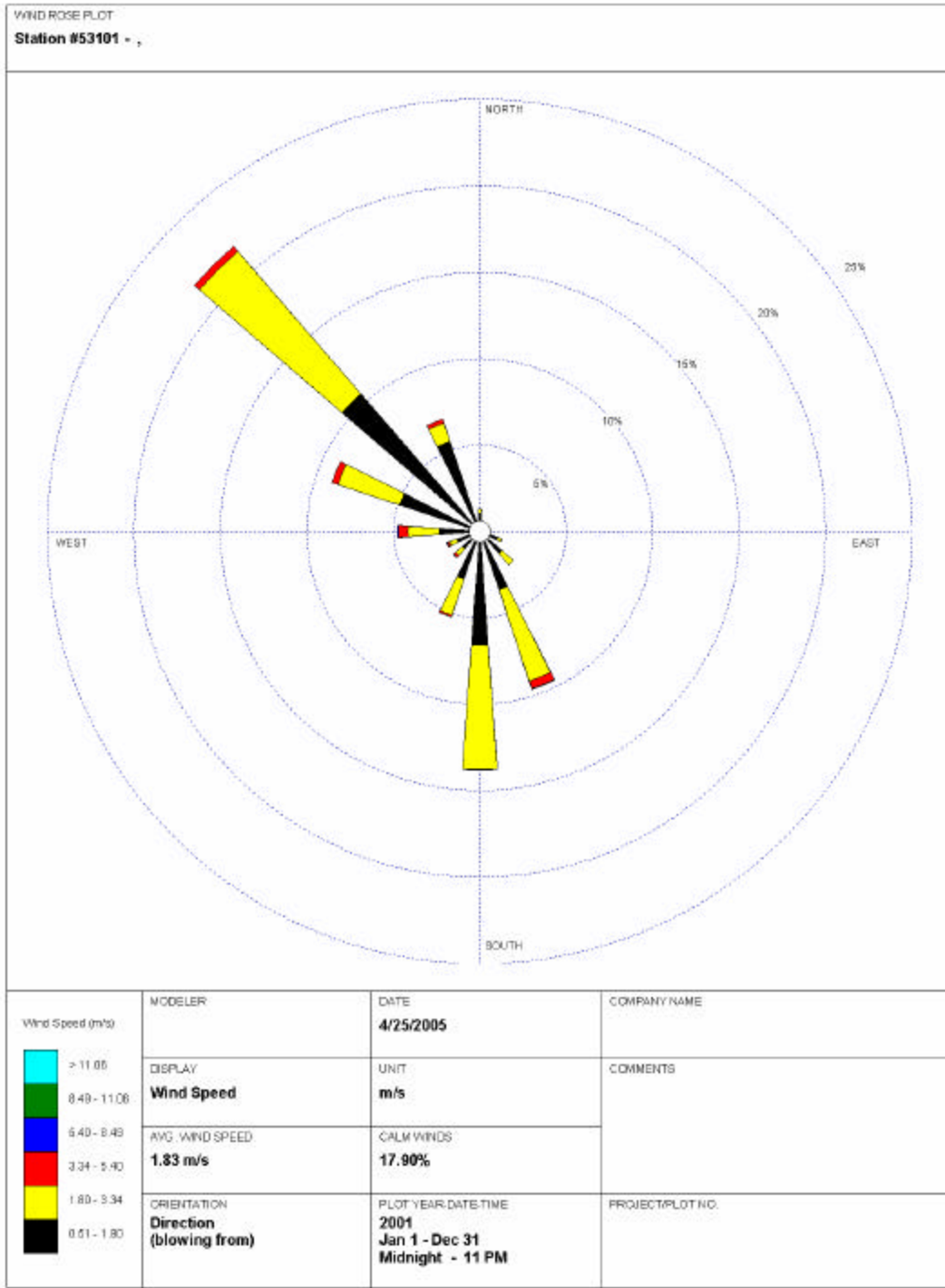
Figure 7: Wind Rose for the Period 1/1/01 to 12/31/01 at the Wilmington Meteorological Site
