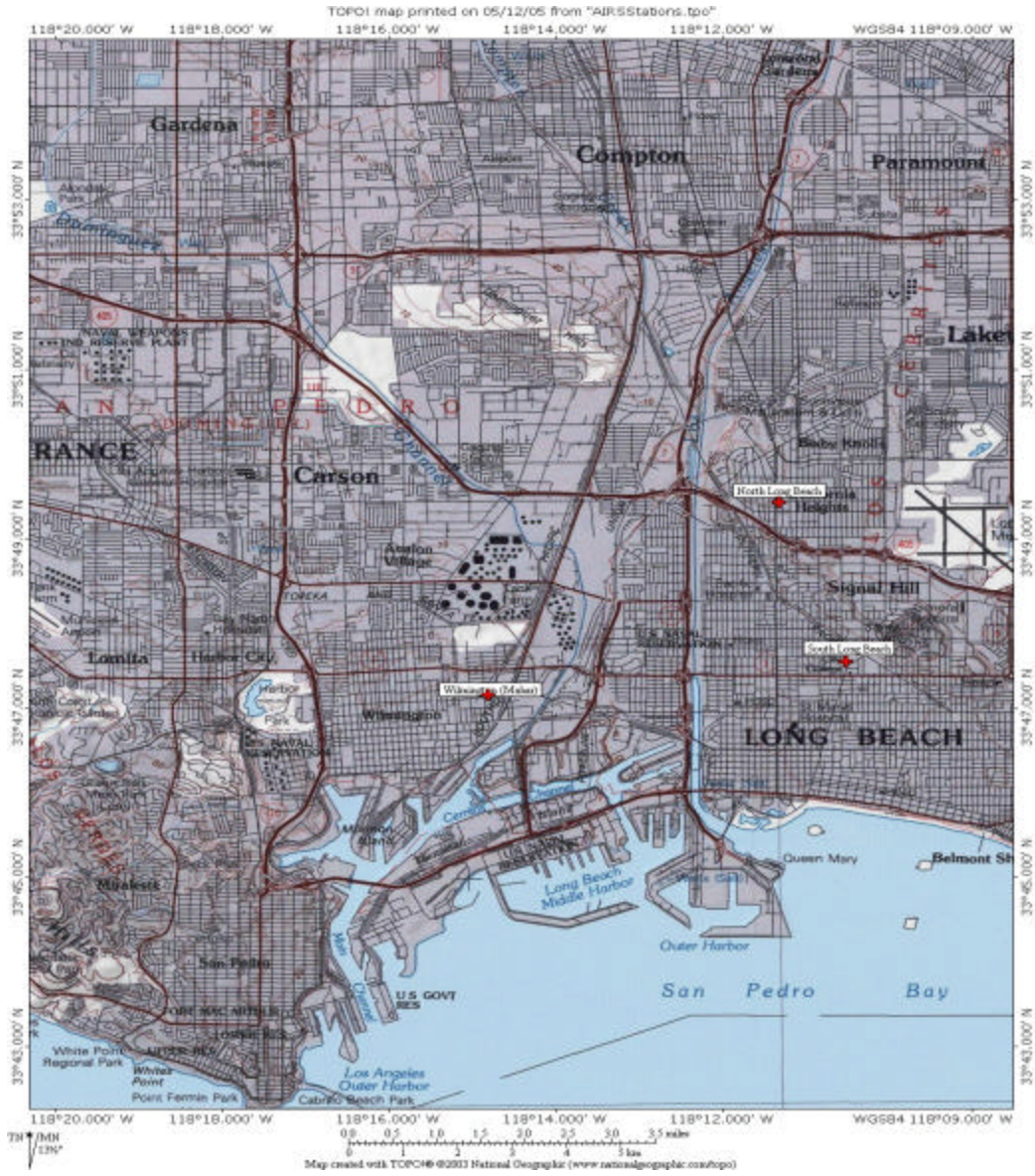
Figure 6: Locations of Surface Meteorological Measurement Sites around the Ports
