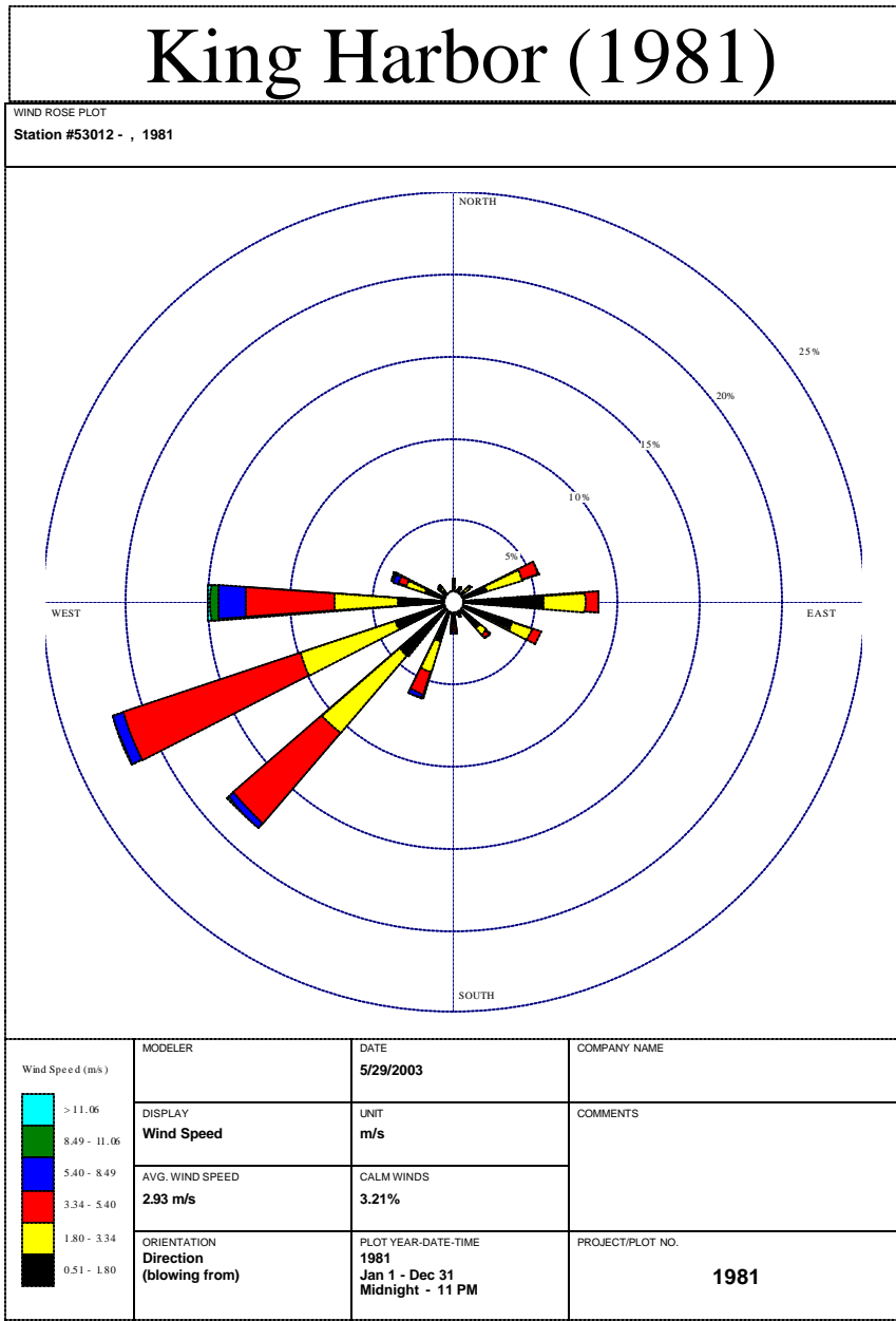
Figure B-2. Wind Rose for King Harbor Meteorological Site
