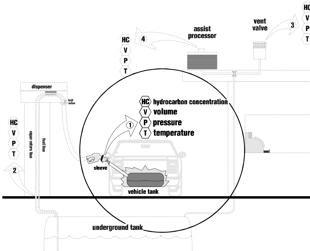
FIGURE 2 Test Point 1 (Nozzle Sleeve)
