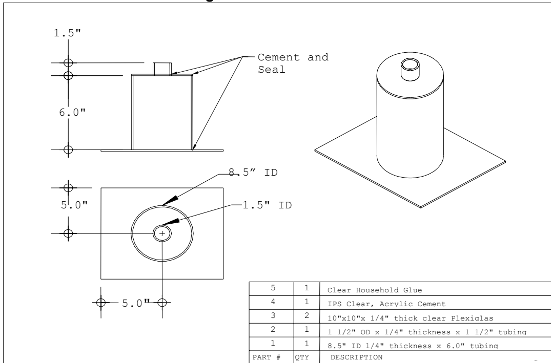
Figure 2. Test Fixture
