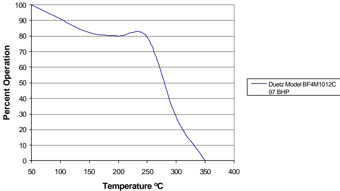
Figure 28: 111624 Exhaust Temperatures Profile Application: Teichert Powerscreen Diesel Generator
