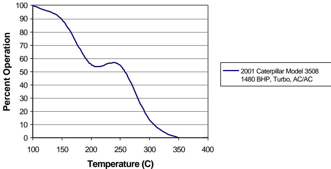
Figure 35: 7810876 Engine Exhaust Temperature Profile Application: Generator Genrig
