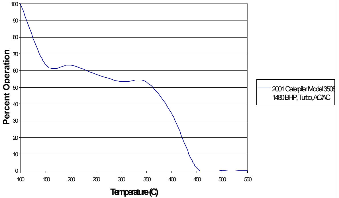
Figure 34: 108739 Engine Exhaust Temperature Application: Drilling Rig Generator
