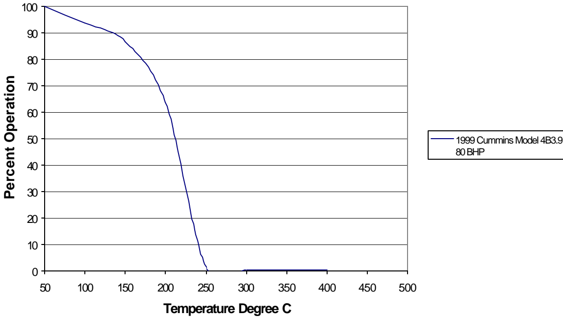
Figure 31: 20022977 Exhaust Temperature Profile Application: Radial Stacker Generator
