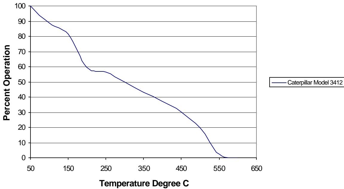
Figure 32: Cecert 43 Exhaust Temperature Profile Application: Rock Crusher Generator
