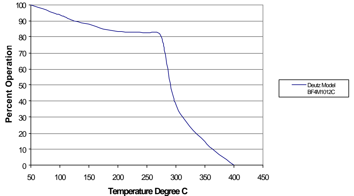
Figure 29: Cecert 14 Exhaust Temperature Profile Application: F.S.T. Sand and Gravel Screening Plant Generator
