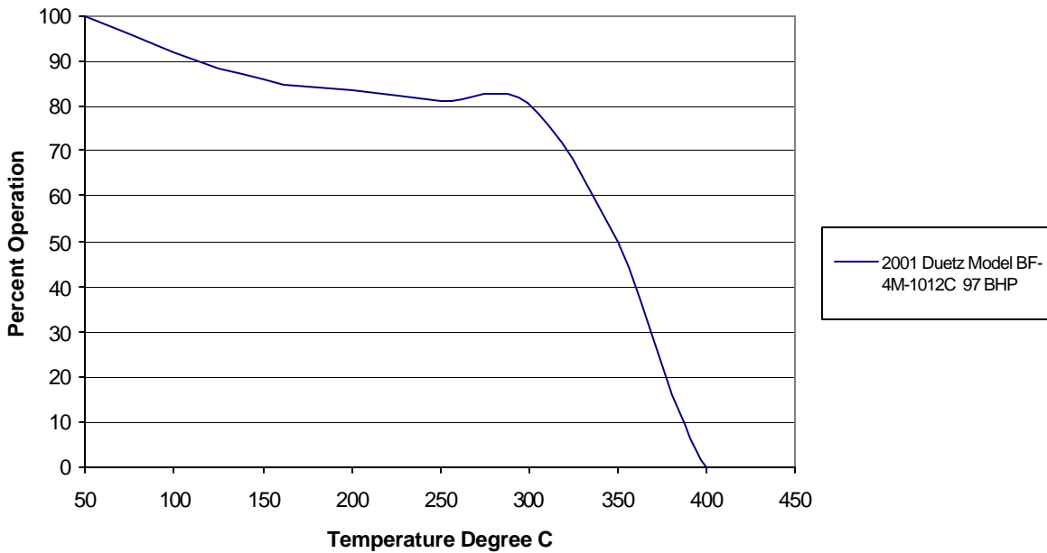
Figure 33: Powerscreen 1800 Exhaust Temperature Profile Application: Screener Generator
