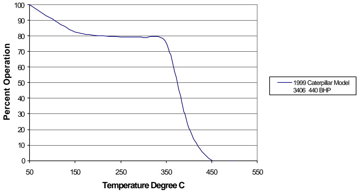
Figure 30: 20004321 Exhaust Temperature Profile Application: Aggregate Recycler Generator
