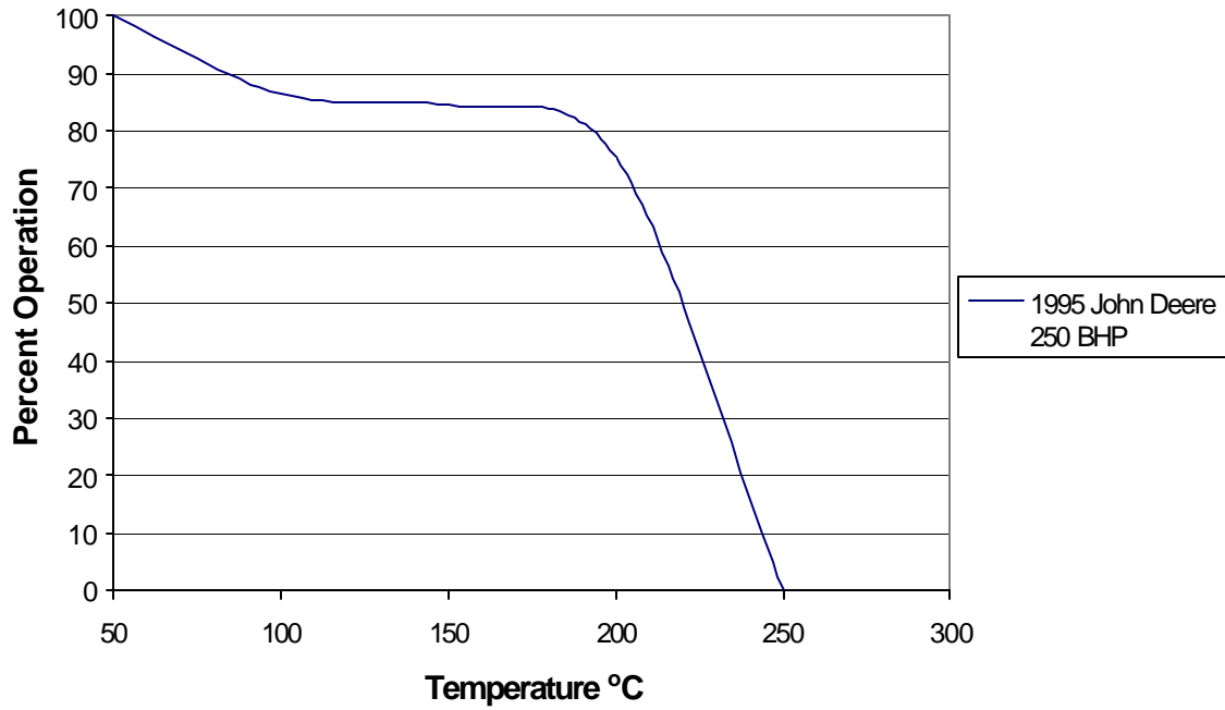
Figure 16: Cecert 36 Exhaust Temperature Profile Application: Lighting Generator
