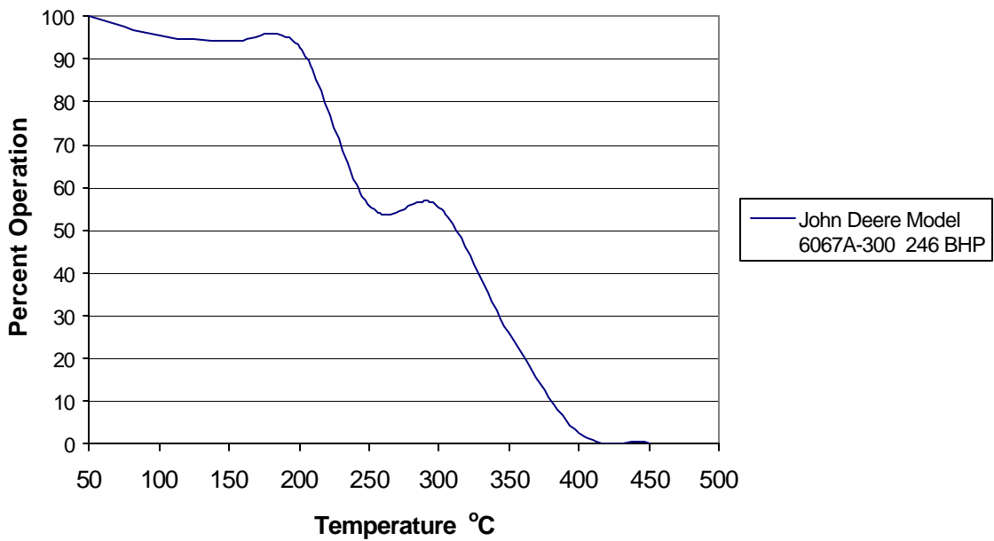
Figure 15: Cecert 34 Exhaust Temperature Profile Application: Lighting Generator
