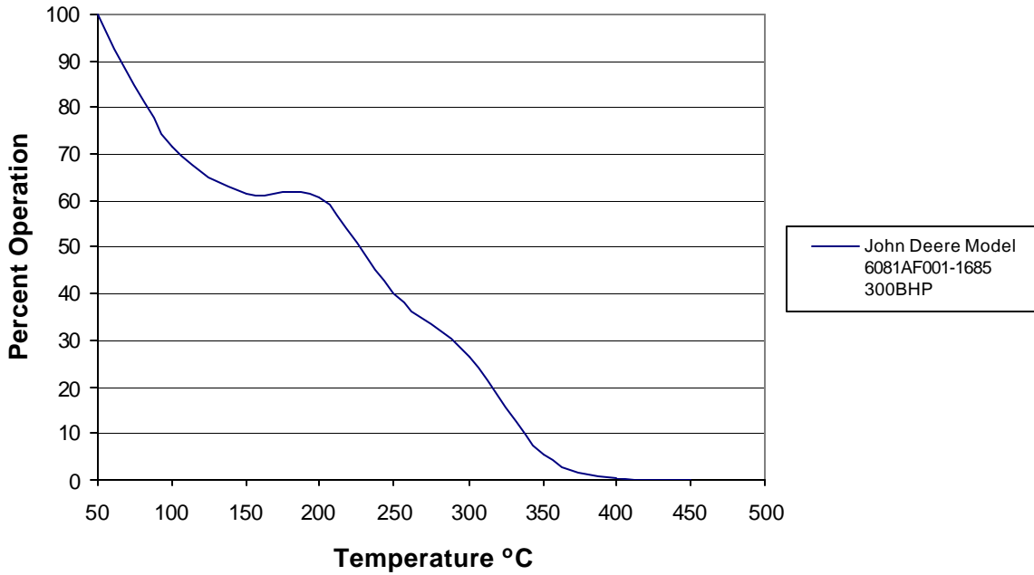
Figure 18: Cecert 38 Exhaust Temperature Profile Application: Lighting Generator
