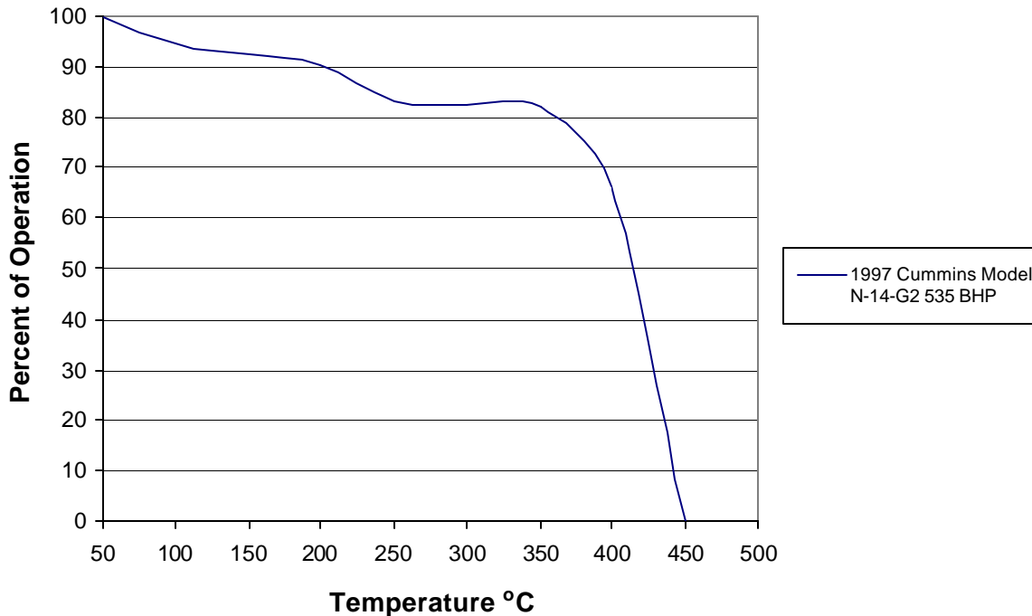
Figure 19: 102261 Exhaust Temperature Profile Application: Conveyor Generator
