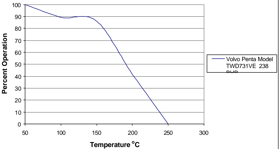
Figure 11: Cecert 29 Exhaust Temperature Profile Application: Rental Generator
