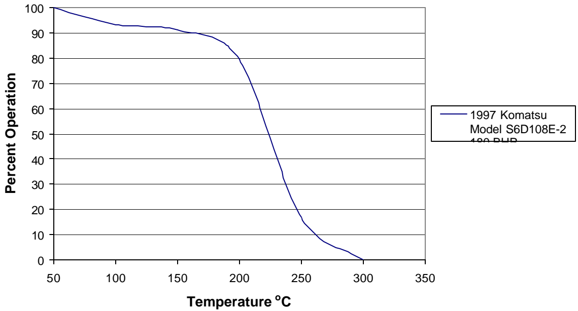
Figure 10: Cecert 28 Exhaust Temperature Profile Application: Rental Generator
