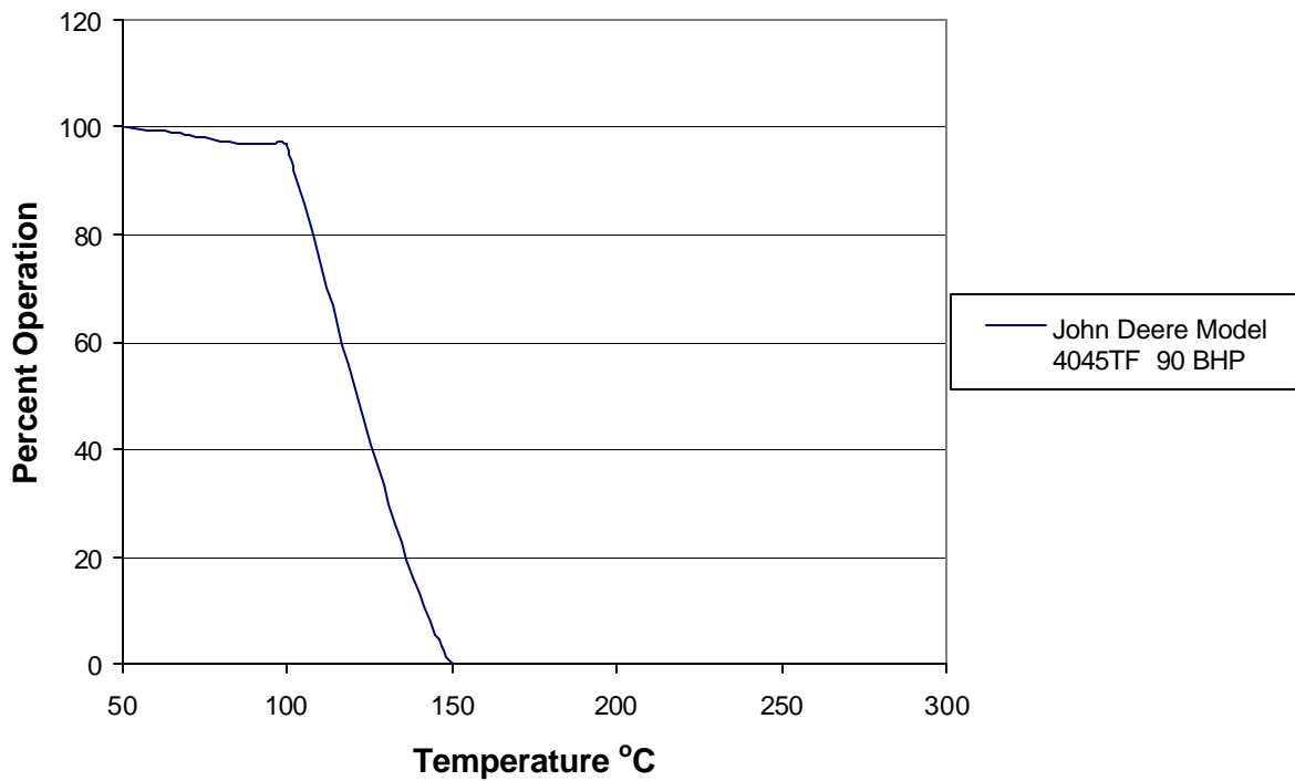
Figure 9: Cecert 27 Exhaust Temperature Profile Application: Rental Generator
