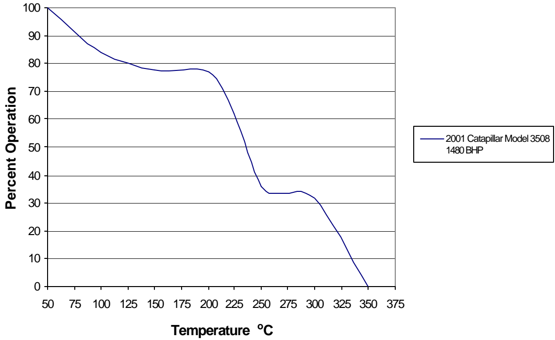
Figure 22: 111223 Exhaust Temperature Profile Application: Rock Crushing & Screening Generator
