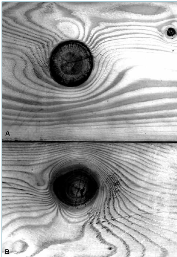
Figure 5–3. Types of knots. A, encased knot; B, intergrown knot.
