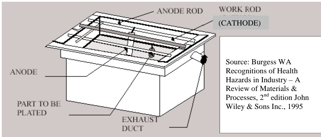
Figure IV-1. Main Components of an Electroplating Tank
