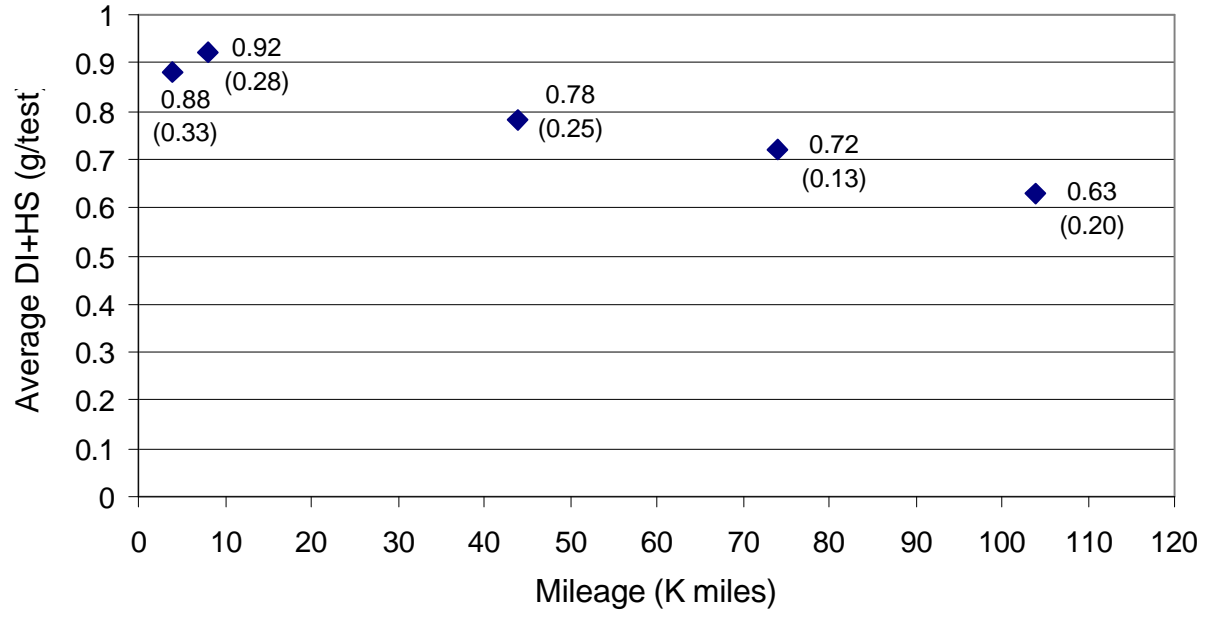
Figure III-4 Nine-Vehicle Crown Victoria Dataset: Average Emissions (Standard Deviation) vs. Mileage
