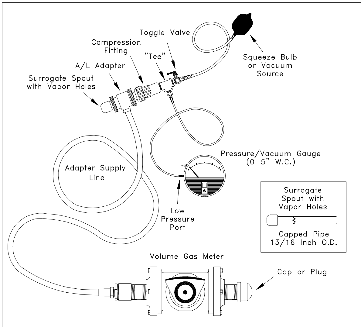
Figure 4 Air To Liquid Adapter Leak Test Assembly
