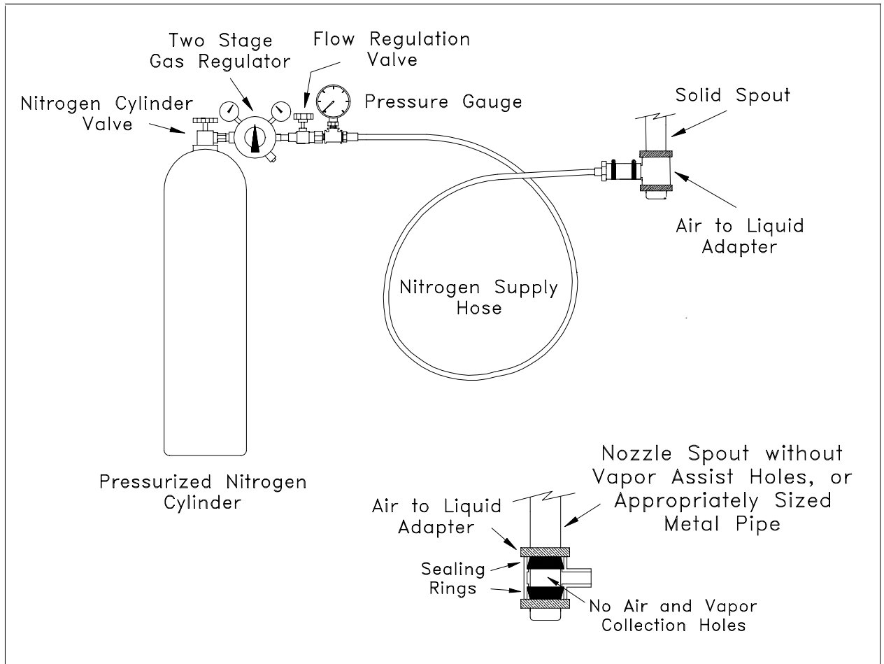
Figure 4 Air To Liquid Adapter Leak Test Assembly
