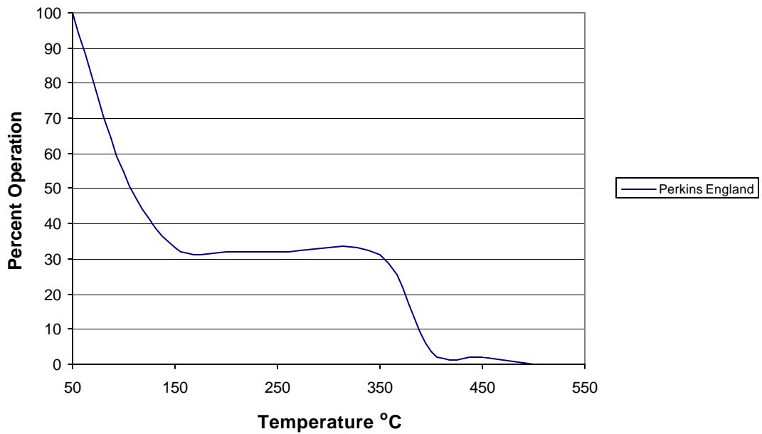
Figure 5: Cecert 24 Exhaust Temperature Profile Application: Chipper
