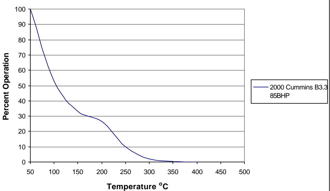
Figure 2: Cecert 17 Exhaust Temperature Profile Application: Chipper
