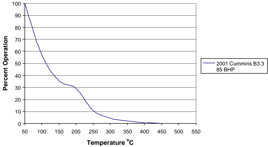
Figure 1: Cecert 16 Exhaust Temperature Profile Application: Chipper
