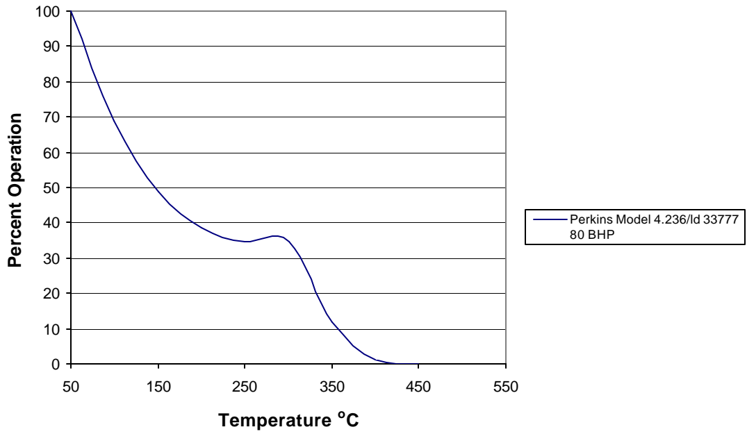
Figure 7: 2526822 Exhaust Temperatures Profile Application: Chipper
