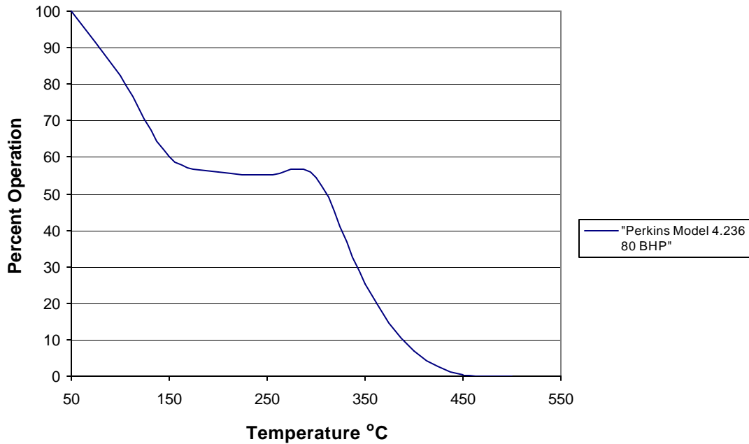
Figure 6: 2526069 Exhaust Temperatures Profile Application: Chipper
