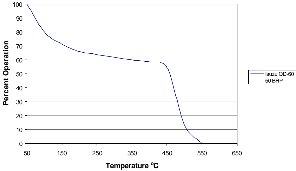
Figure 48: Cecert 45 Exhaust Temperature Profile Application: Compressor
