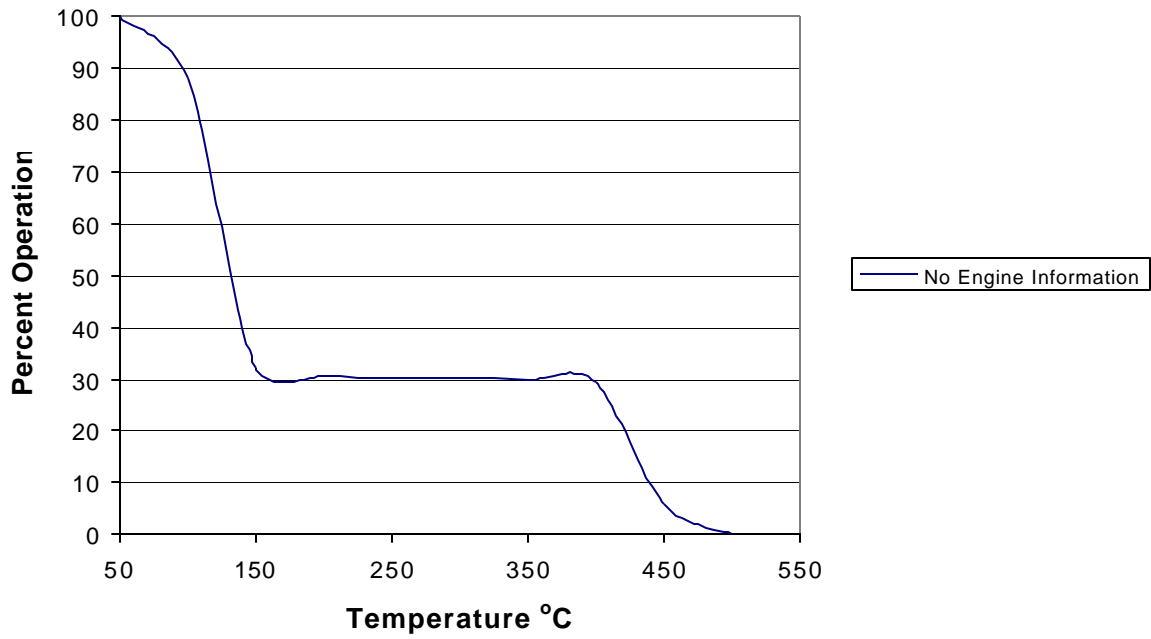
Figure 44: Cecert 25 Exhaust Temperatur Profile Application: Compressor
