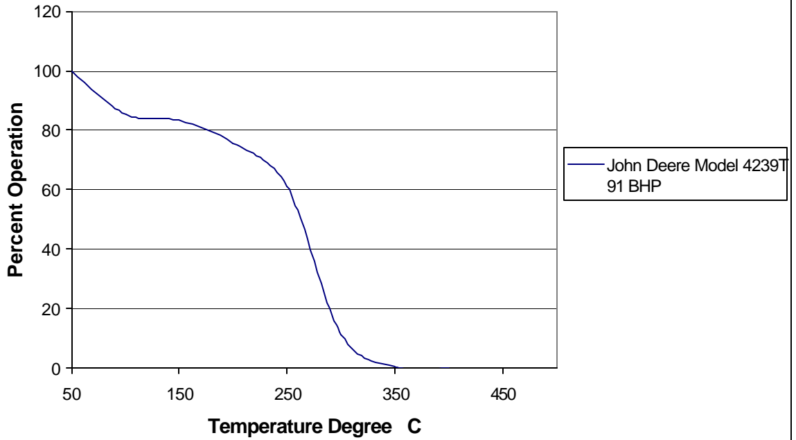
Figure 36: 0534128 Exhaust Temperature Profile Application: Paint Striper Compressor
