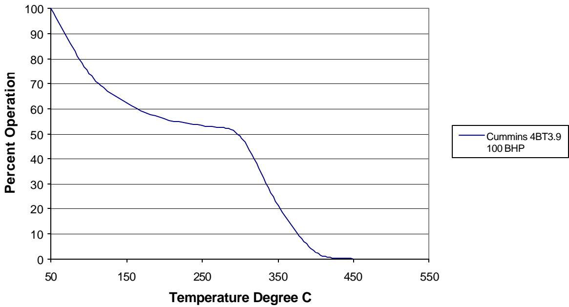
Figure 46: 2715368 Exhaust Temperature Profile Application: Compressor
