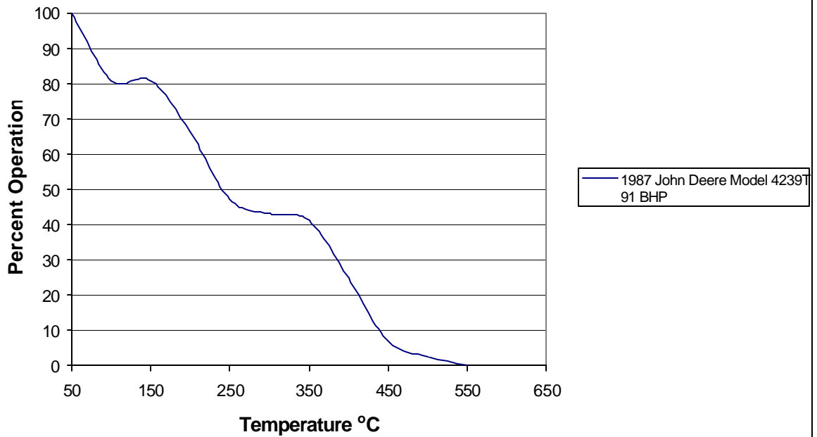
Figure 37: Cecert 1 Exhaust Temperatures Profile Application: Paint Striper Compressor
