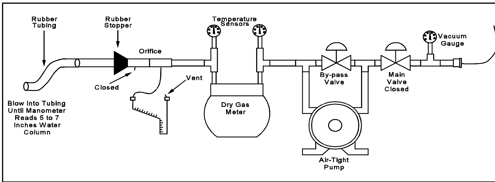
Figure 17-5. Leak Check of Meter Box.
