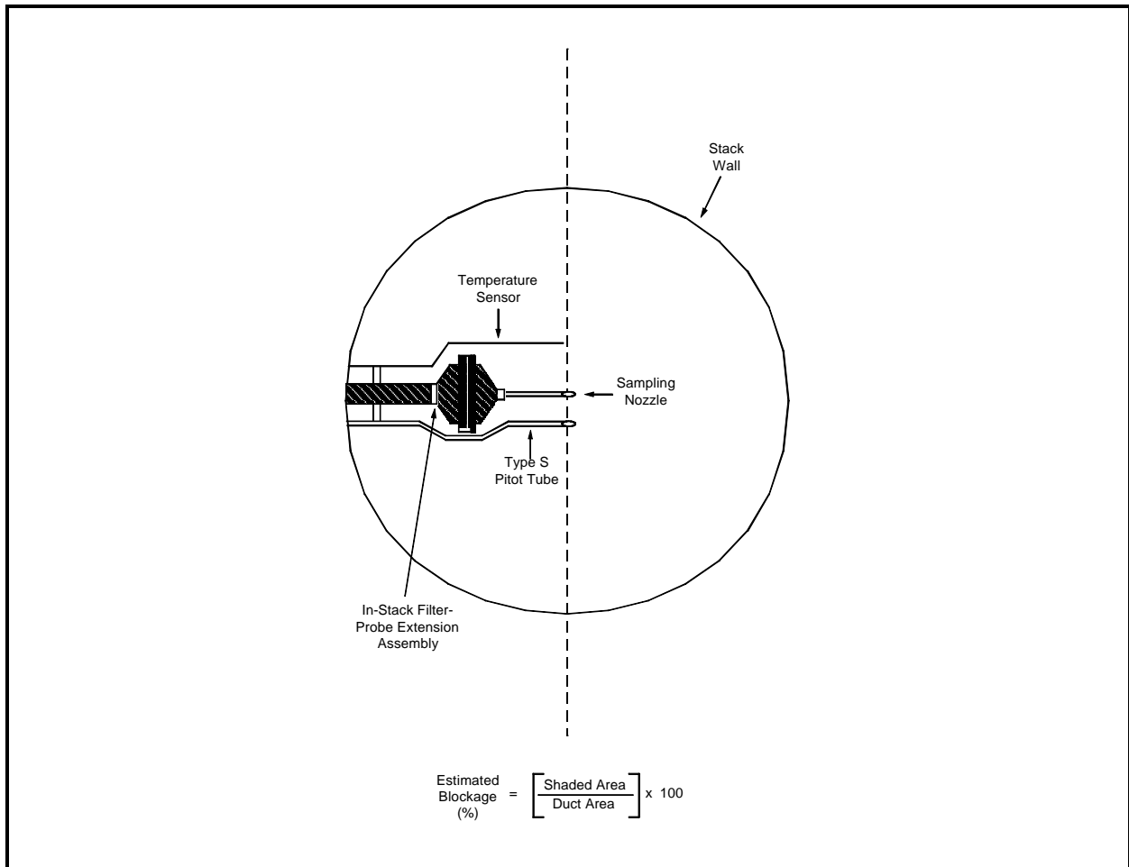
Figure 17-2. Projected-area model of cross-section blockage (approximate average for a sample traverse) caused by an in-stack filter holder-probe extension assembly.
