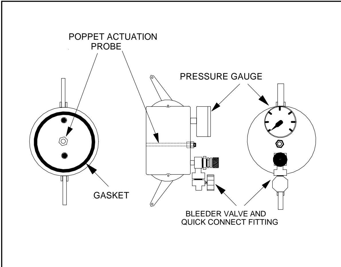
Figure 3 Vapor Coupler Test Assembly
