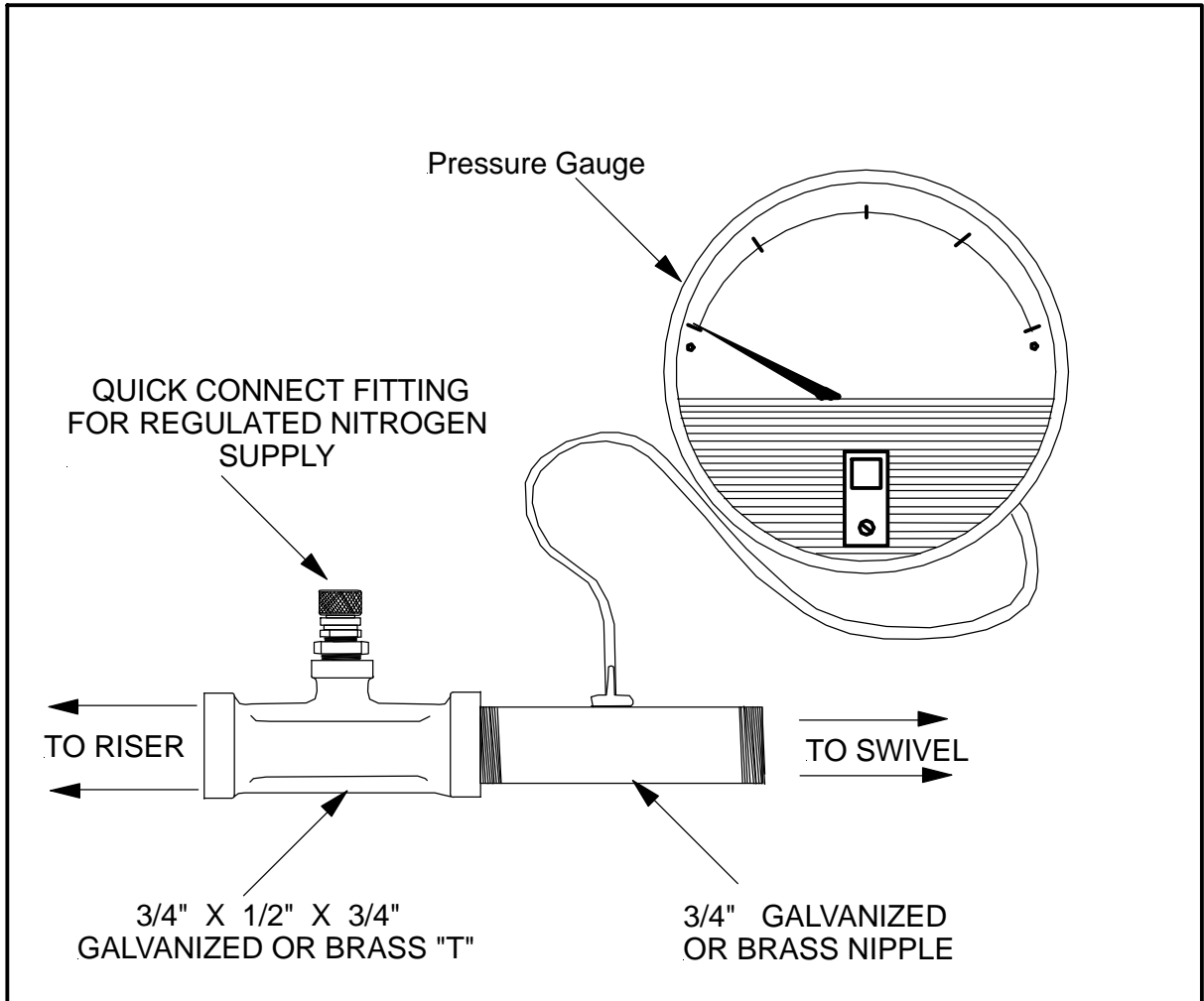
Figure 1 "T" Connector Assembly
